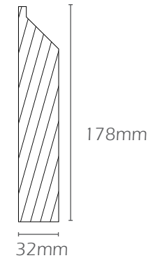
Skirting/Starter Board
