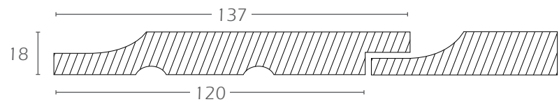
Rebated Shiplap
