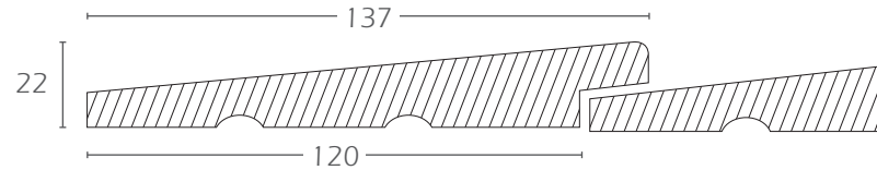
Rebated Bevel 6
