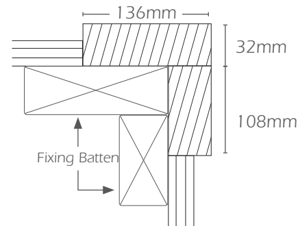
Two Piece Corner (32mm x 108mm x 32mm x 136mm)
