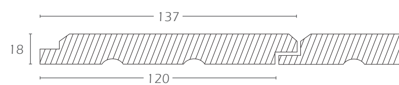
Rebated V-Joint
