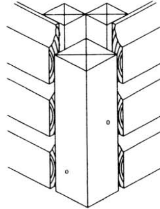
1-piece External
