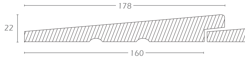
Rebated Bevel 8
