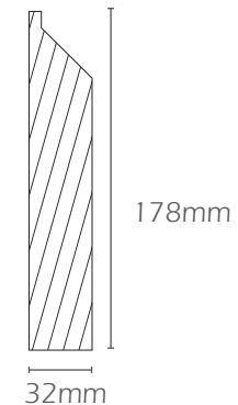
Skirting/Starter Board
