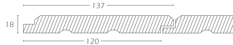
Rebated V-Joint
